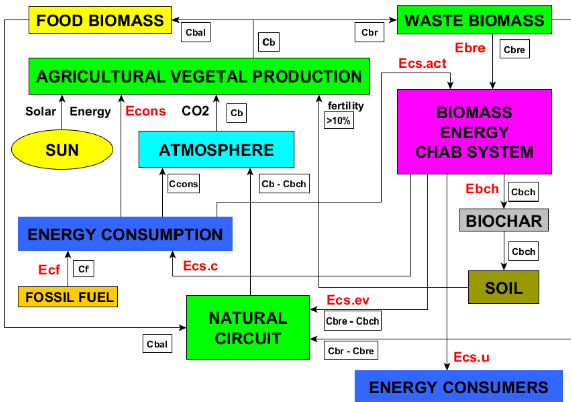
Fig. 3. Model of biomass energy system with CHAB concept
